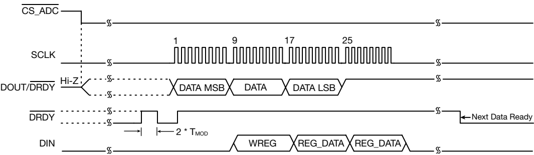
Figure 3-1. ADC Communciations and Initialization
