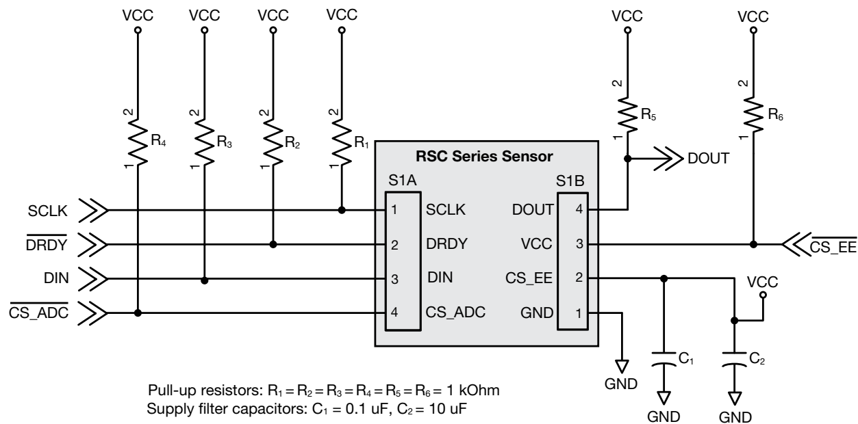
Figure 6. Recommended Circuit
