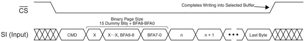
Figure 24-2. Buffer Write
