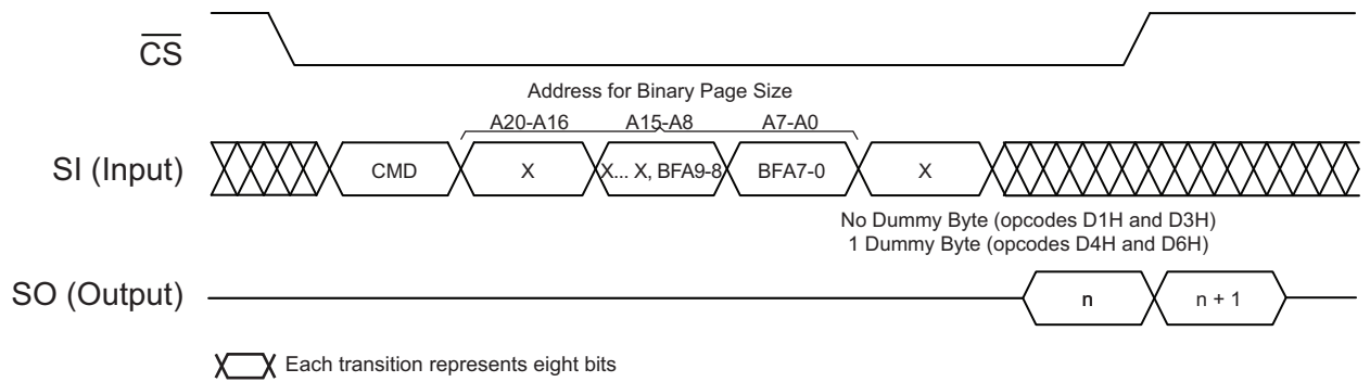
Figure 25-4. Buffer Read
