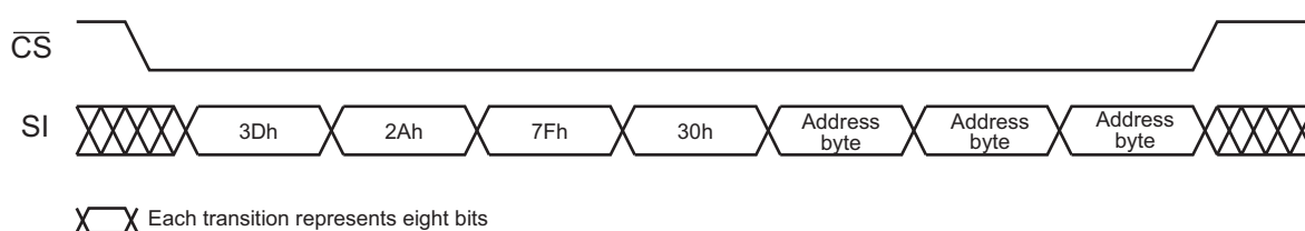
Figure 9-1. Sector Lockdown
