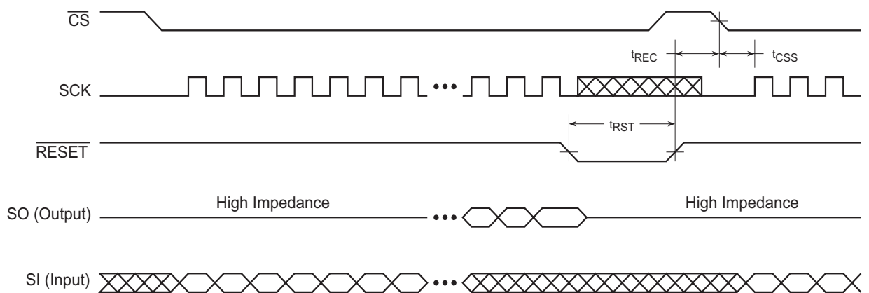
Figure 26-12. Reset Timing
