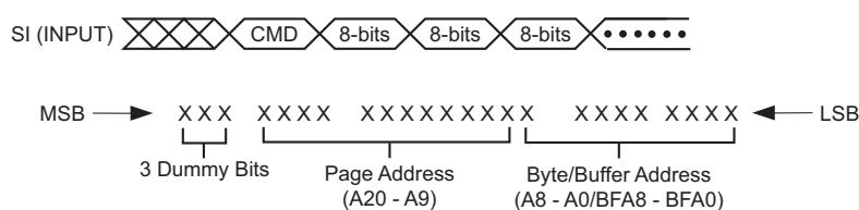
Figure 22-2. Command Sequence for Read/Write Operations for Page Size 512 bytes (Except Status Register Read, Manufacturer and Device ID Read)
