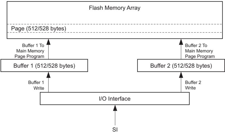
Figure 24-1. Block Diagram
