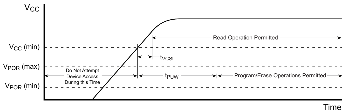
Figure 17-1. Power-Up Timing
