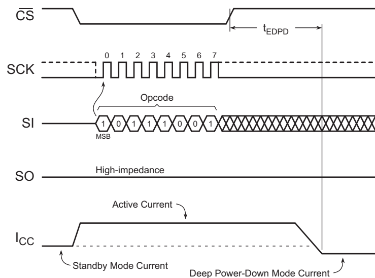
Figure 11-1. Deep Power-Down Timing
