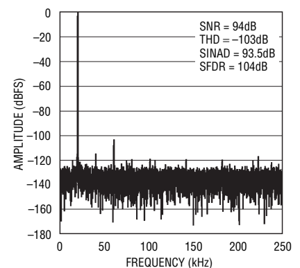
16k Point FFT f_s = 500\text{ksps} , f_{\text{IN}} = 20\text{kHz}
