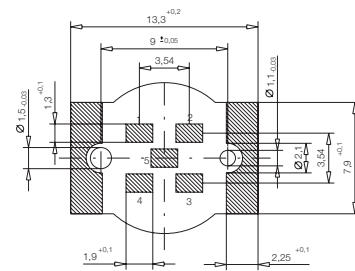
Layout for connectors with machined contacts
