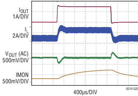
Load Step (Buck-Boost Region – Figure 37)
