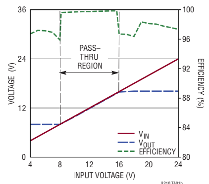
Pass-Thru Transfer Characteristic ( V_{OUT(BOOST)} = 8\text{V} , V_{OUT(BUCK)} = 16\text{V} )
