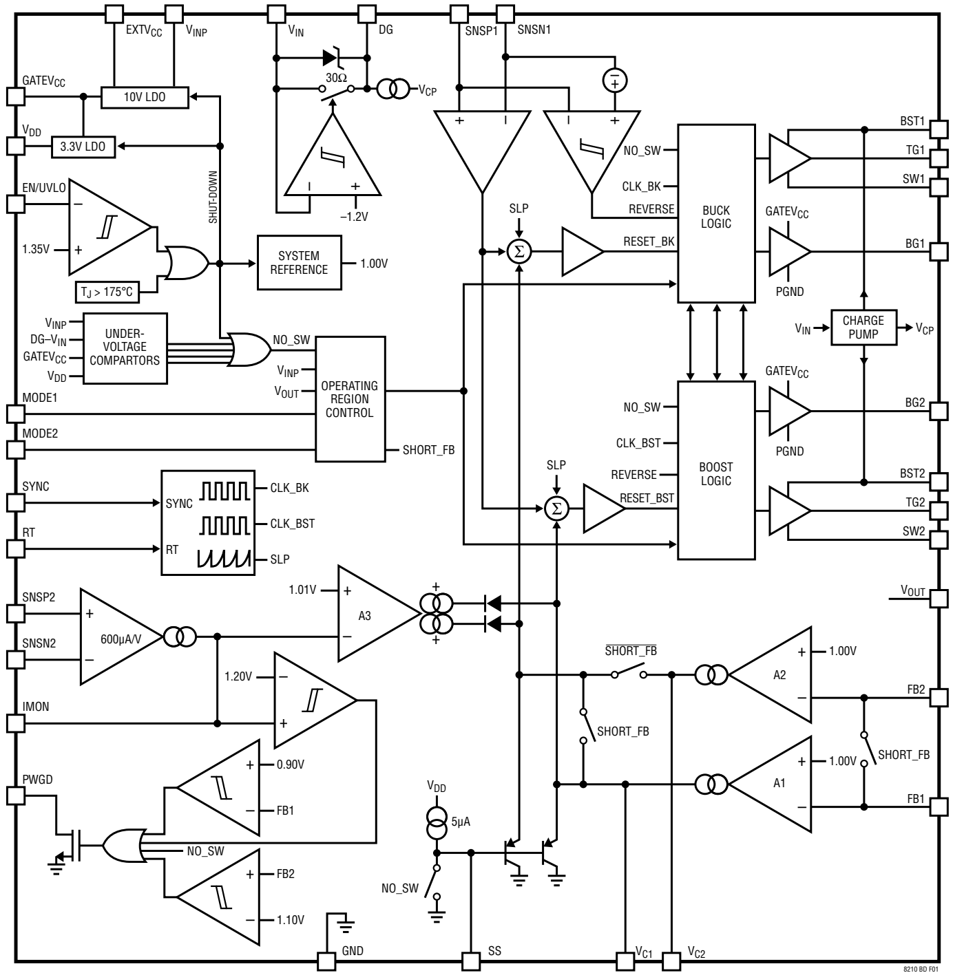
Figure 1. Block Diagram
