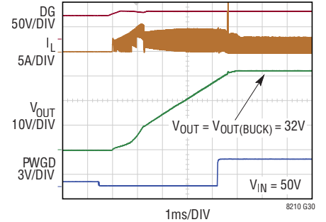
Pass-Thru Start-Up: V_{IN} Above Pass-Thru Window (Figure 38)
