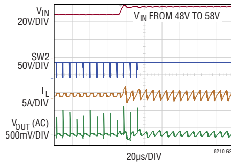
Line Step (Buck-Boost Region – Figure 37)
