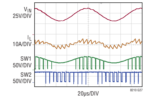
High Frequency Switching Region Transitions (CCM Mode – Figure 37)
