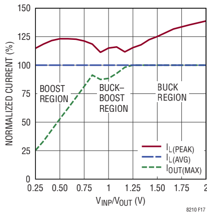
Figure 17. Example of Maximum Average Inductor Current and Output Current vs V_{INP}/V_{OUT}
